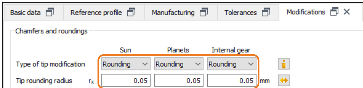
Figure 25. Tip modification «rounding» the tooth form
