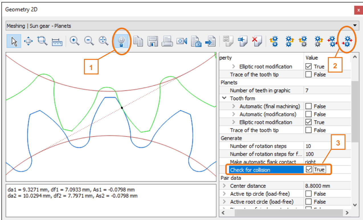
Figure 29. Activating collision check and displaying pair 1
