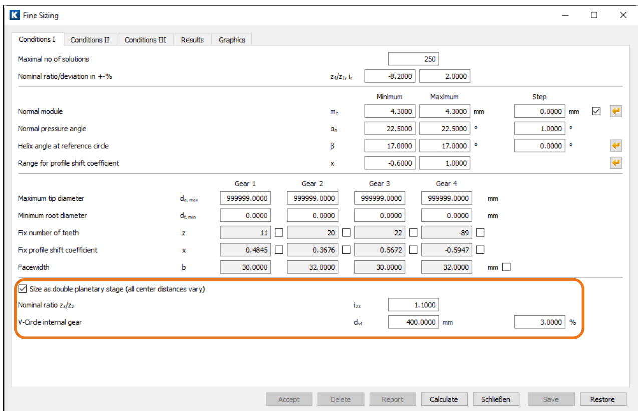
Figure 31. double pinion planetary stage in the Fine Sizing
