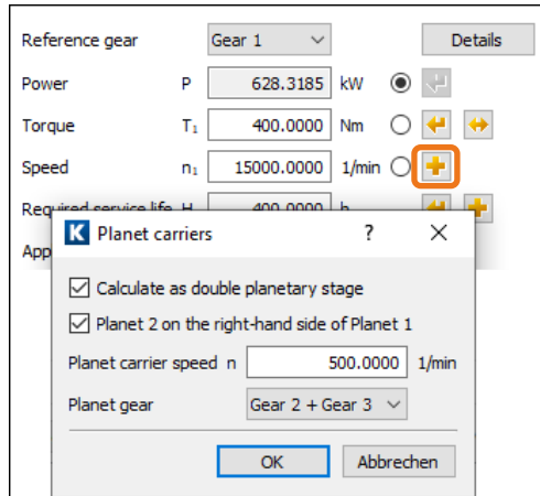
Figure 30. Planet carrier in the Four gears train module
