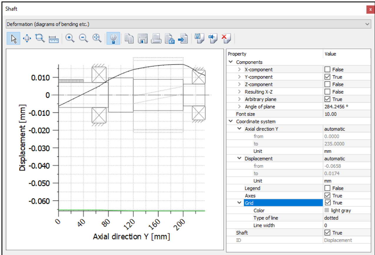
Figure 9. Display produced by selecting the Displacement option
