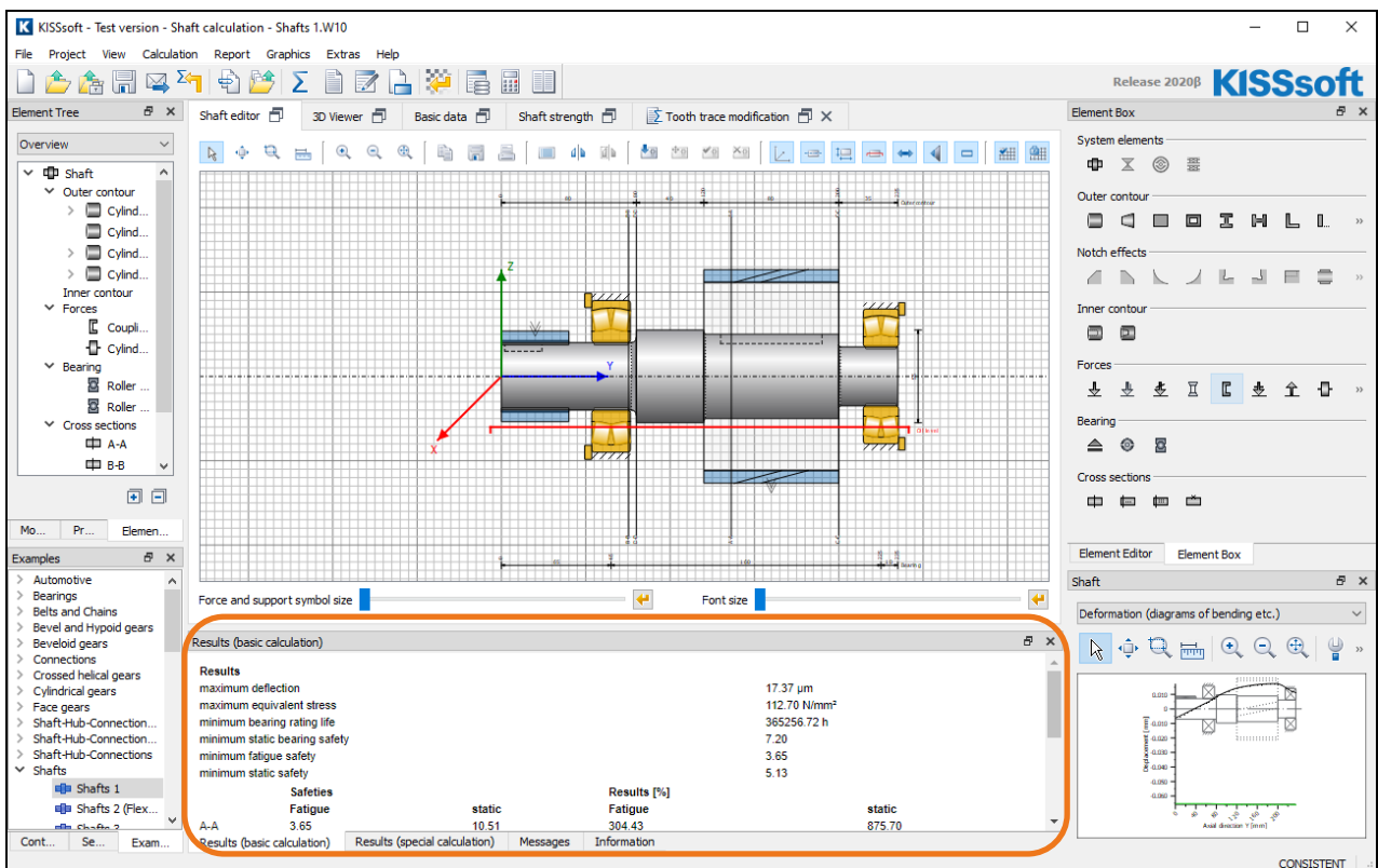
Figure 5. Opened shaft analysis
